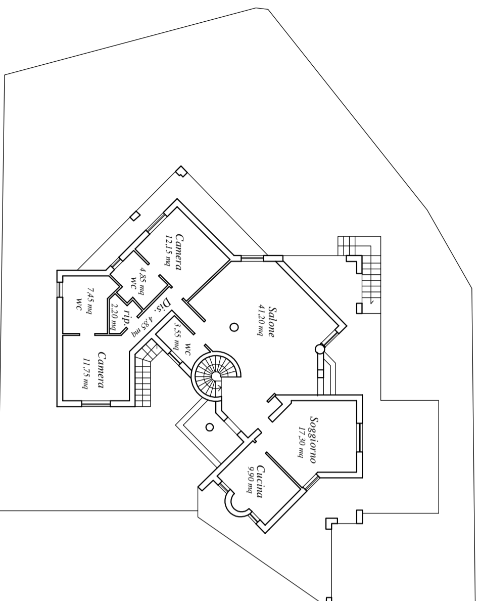
Piano Terra
